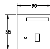
CONVECTION CURRENTS
