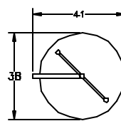
HYPERBOLIC SLOT
