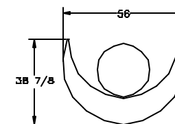
STRANGE ATTRACTOR
