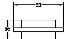
CHAOTIC PENDULUM
