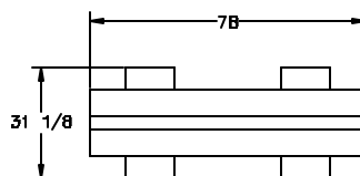
NON-ROLLING ROLLERS
