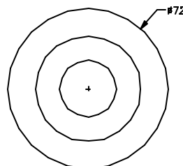
CLOUD RINGS
